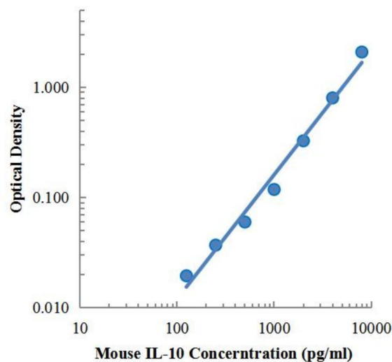
Mouse IL-10 Typical Standard
